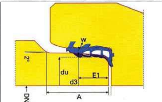
SEALING RING BETWEEN CONCRETE PIPES
